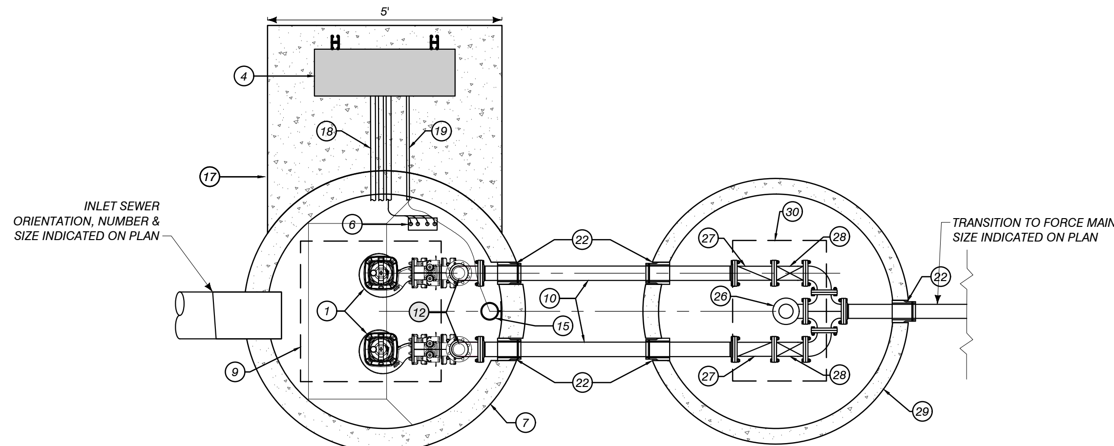
LIFT STATION PLAN VIEW
