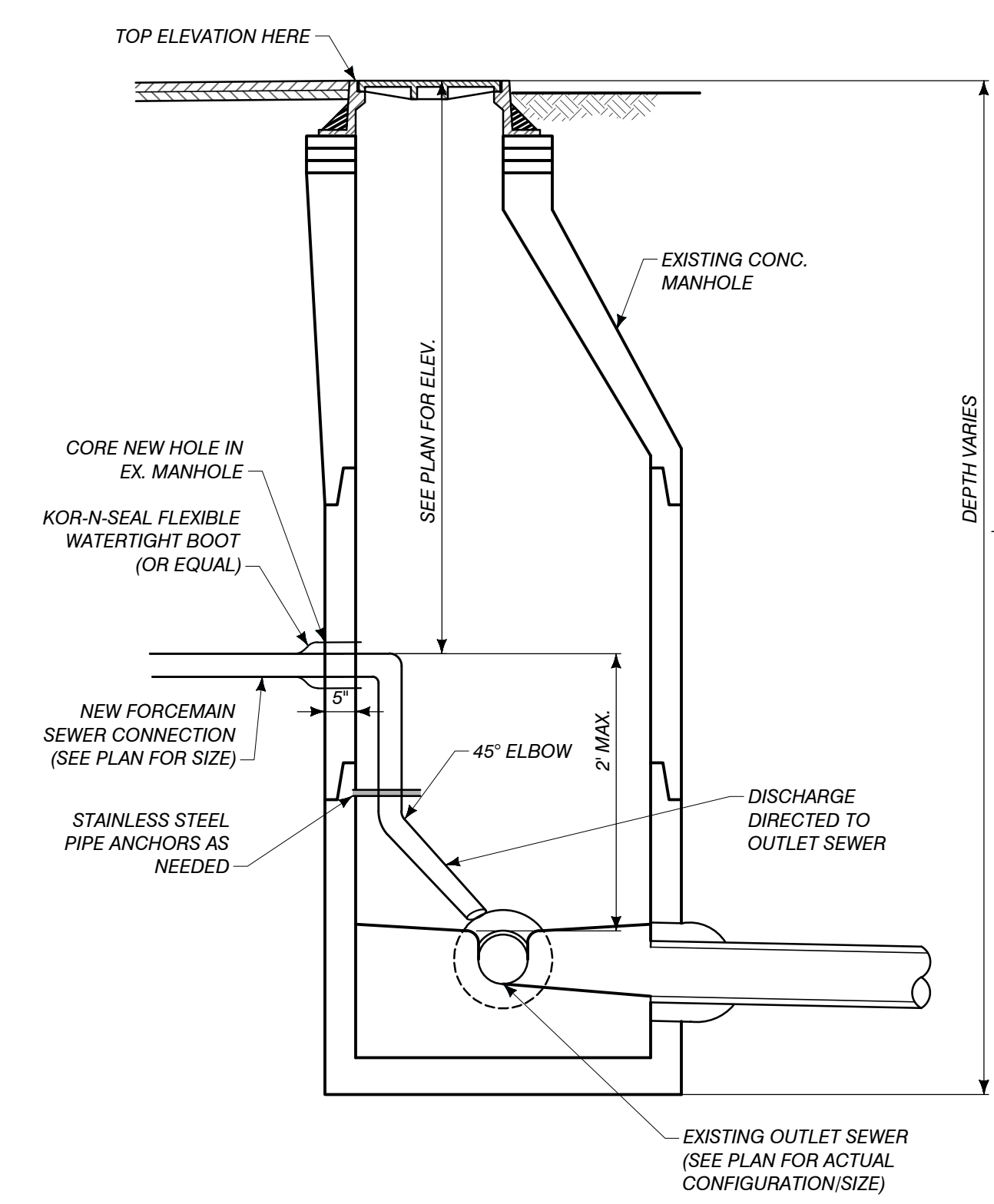
EXISTING SEWER TIE-IN DETAIL
