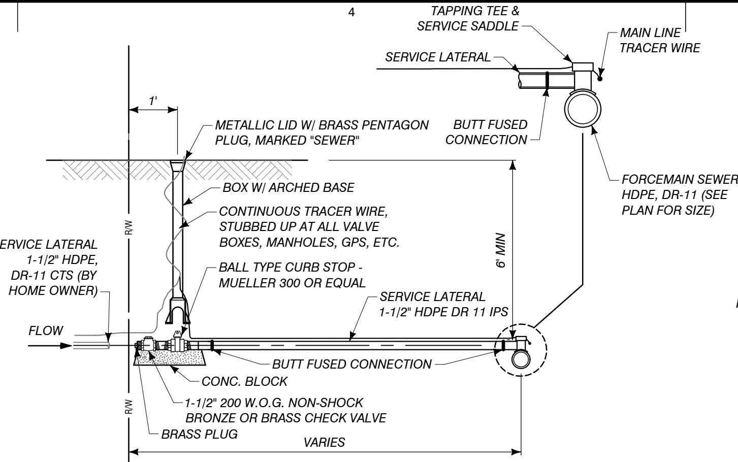
PRESSURE SERVICE DETAIL
