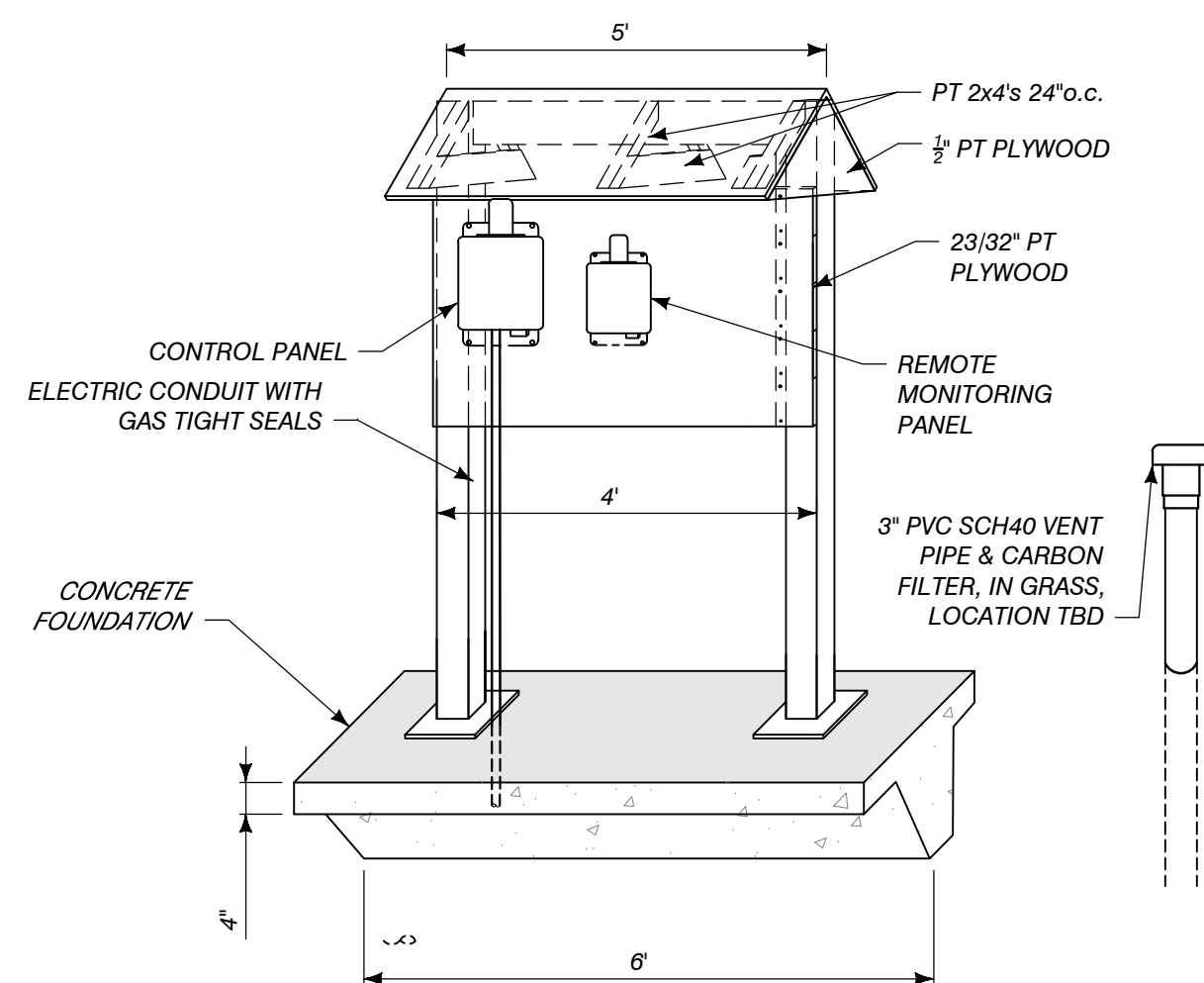
FRONT VIEW
