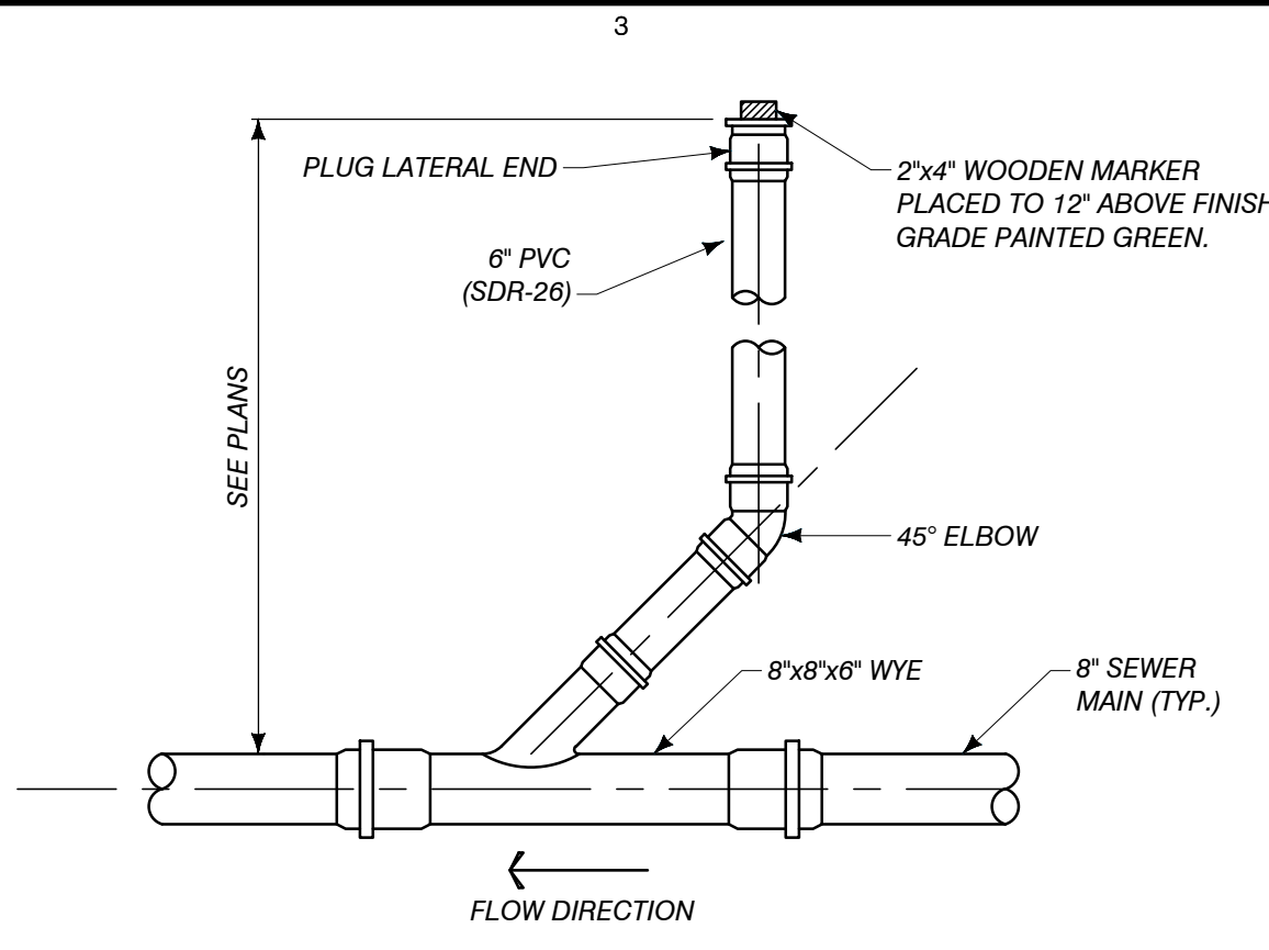
GRAVITY SERVICE DETAIL
