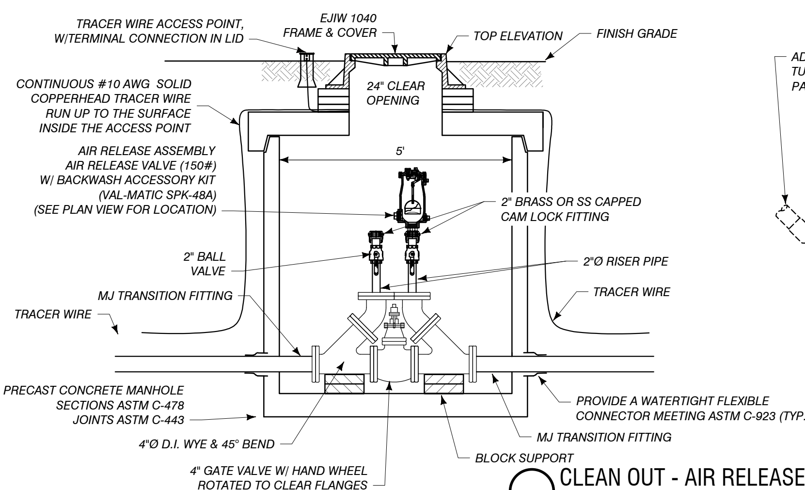
CLEAN OUT - AIR RELEASE
