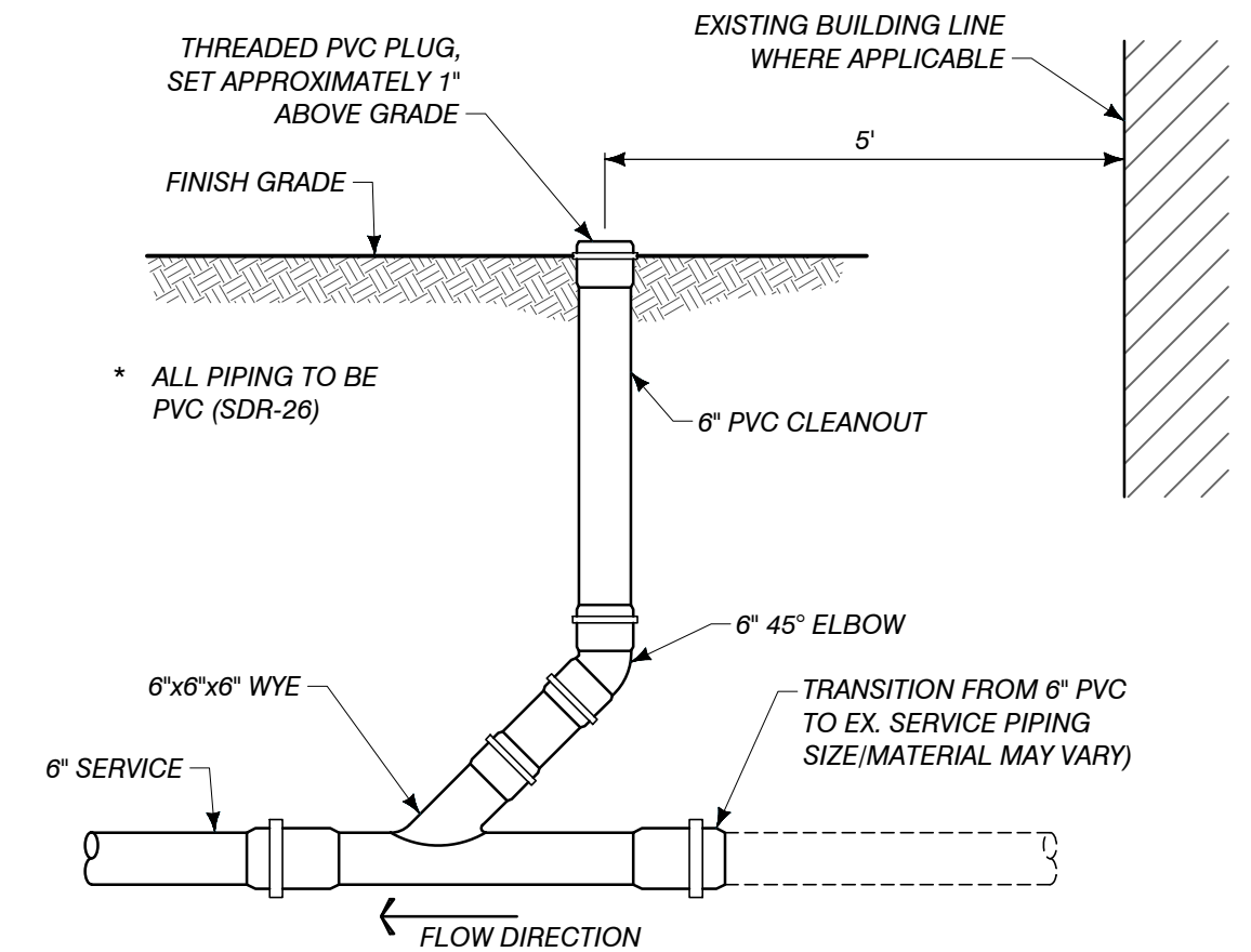
GRAVITY SERVICE CLEANOUT DETAIL
