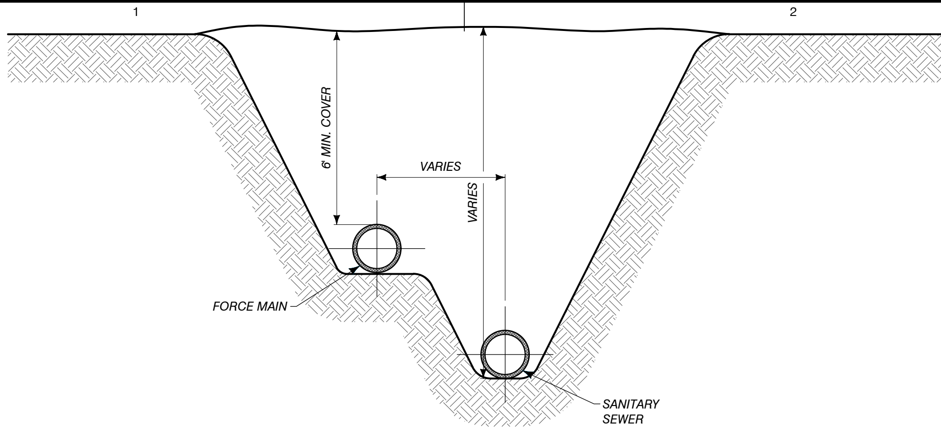
2 PIPE TRENCH DETAIL
