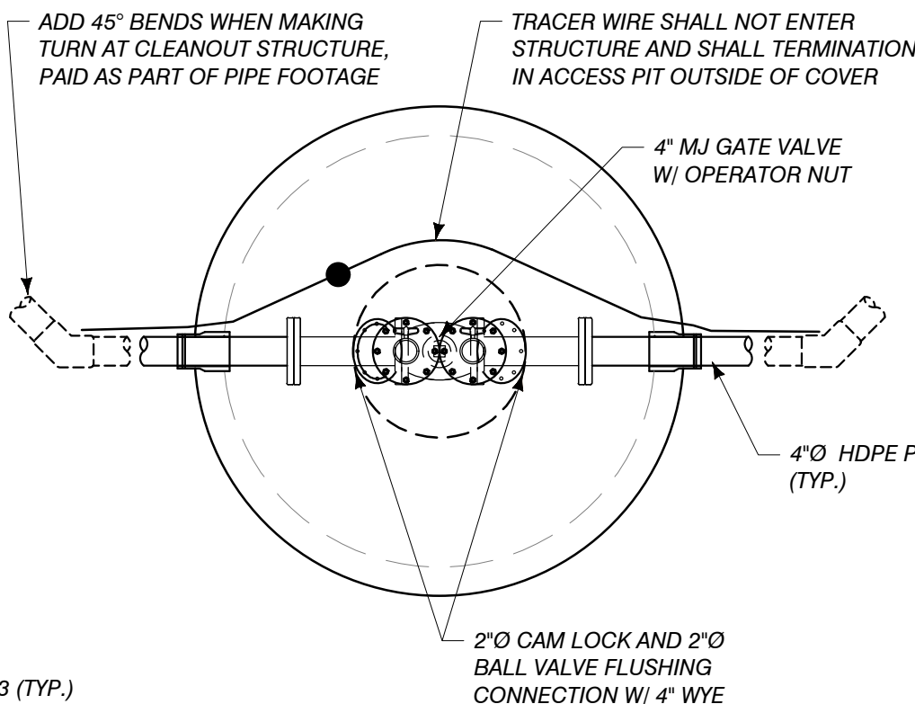
EXISTING SEWER TIE-IN DETAIL
