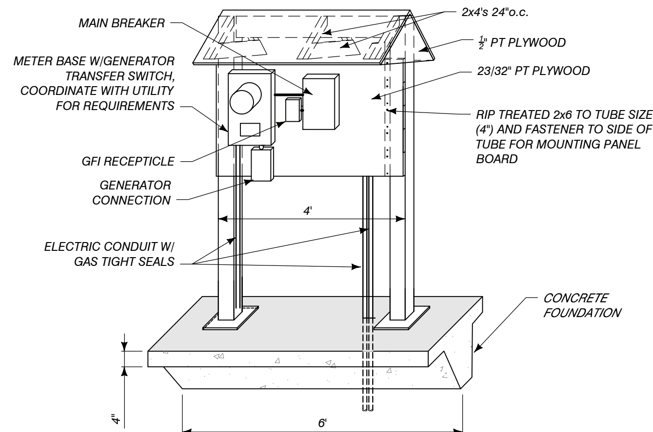
REAR VIEW
