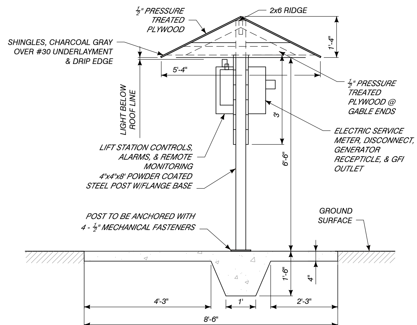
SIDE VIEW
