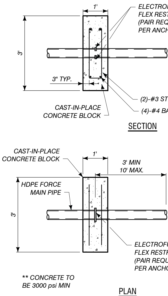
HDPE FORCE MAIN ANCHOR DETAIL
