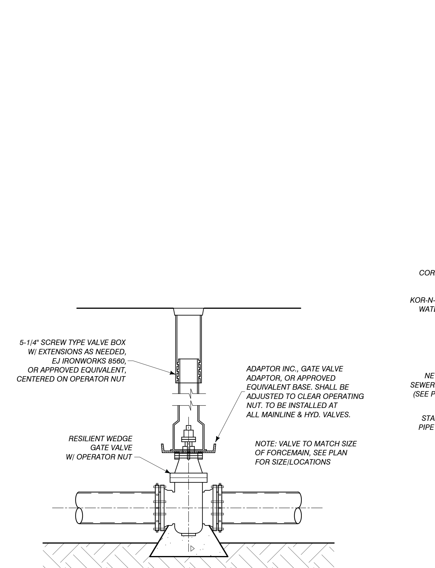
FORCEMAIN VALVE & BOX DETAIL
